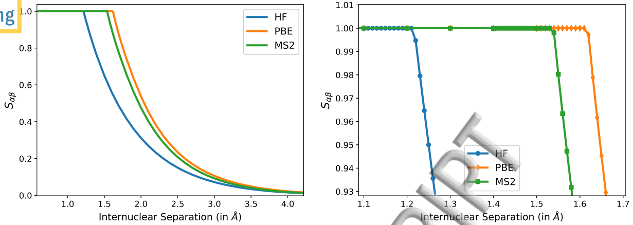
FIG. 10: Overlap S_{\alpha\beta} predicted by three ‘qualitatively acceptable’ methods (HF, PBE and MS2) for stretched H_2 , highlighting a constant plateau till the CF point, followed by exponential decay (left). The right panel shows the behavior close to the CF point, highlighting a clear derivative discontinuity for all three methods.
