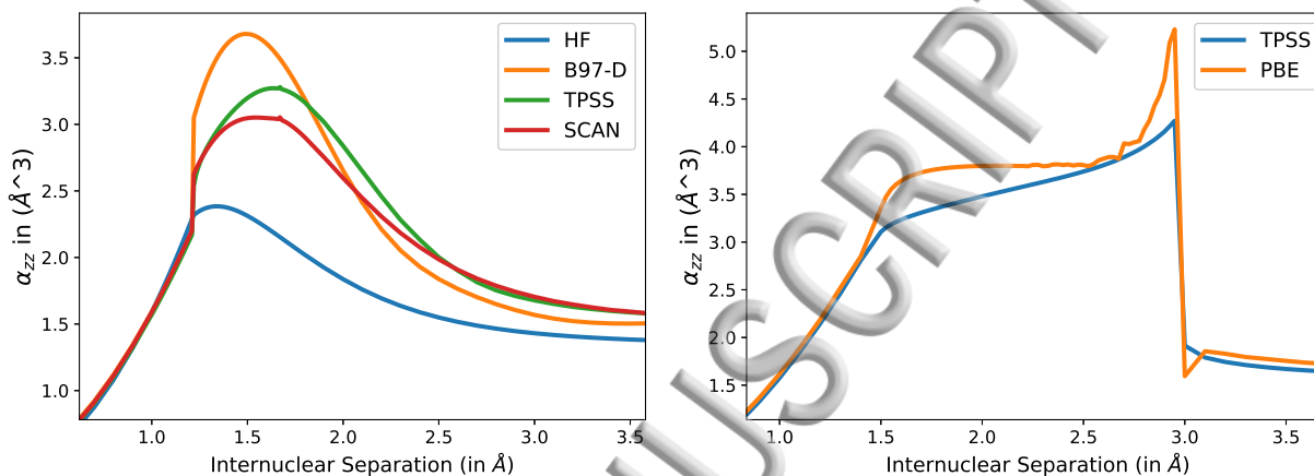
FIG. 13: Static polarizability parallel to the bond axis generated from HF orbitals (left) and TPSS orbitals (right).
